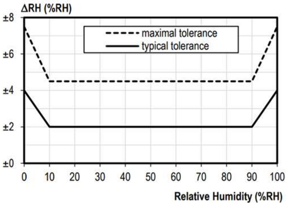
Figure 1 : Tolerance of RH at 25°C for DL-100TMS-ZT
