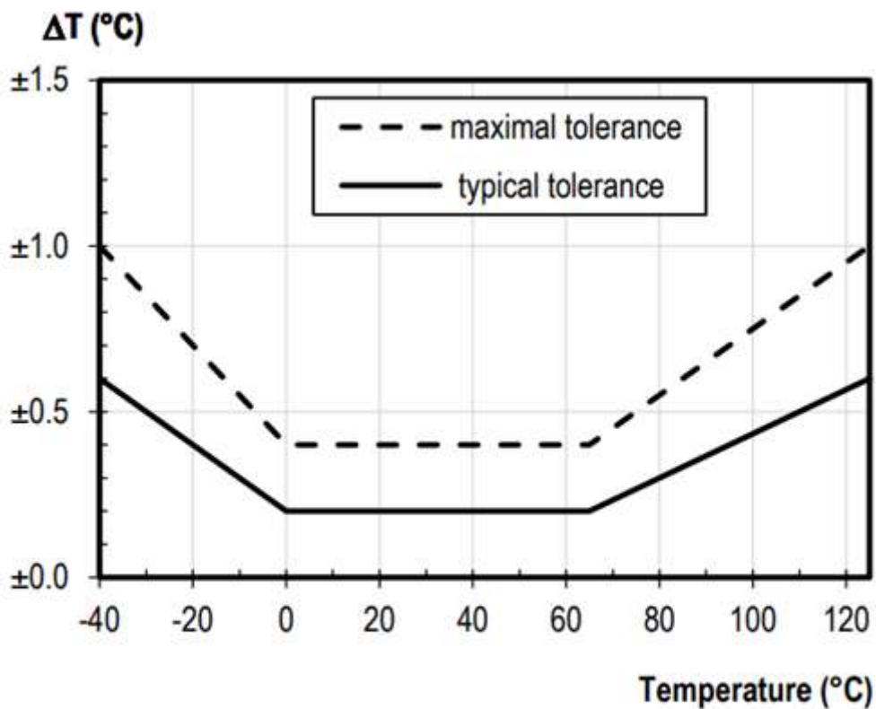
Figure 2 : Temperature accuracy of DL-100TMS-ZT
